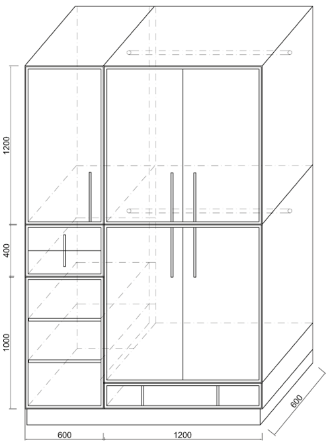
Sample scheme of the Riddle Modular System.
